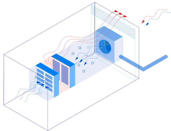
Evaporative Cooling
