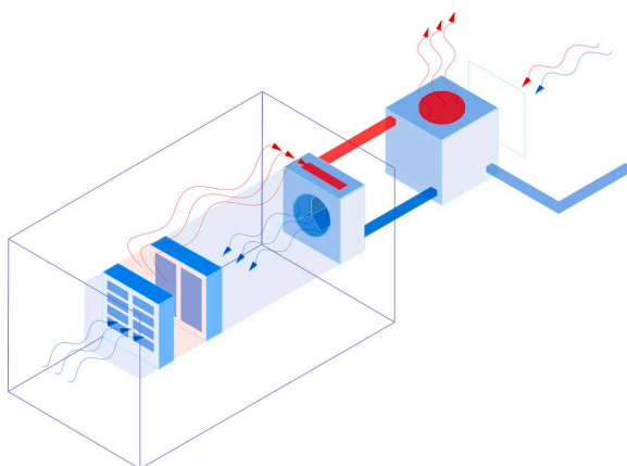
Adiabatic Cooling
