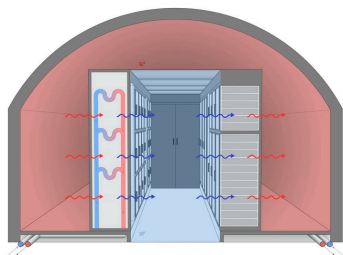
Serverroom
